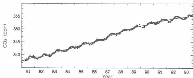
Fig. 2.5. \text{CO}_2 data and long-term trend for SPO. Note that the 1992-1993 growth rate decline is not as pronounced as at Mould Bay.
