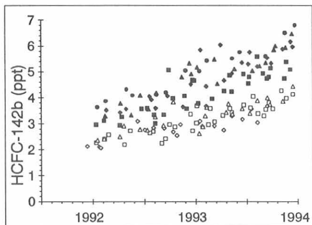
Fig. 5.9. Mixing ratios determined for HCFC-142b from air collected in flasks from seven different remote sampling locations: Alert, (•); BRW, (▲); Niwot Ridge, (◆); MLO, (■); SMO, (Δ); CGO, (□); and SPO, (◇).
