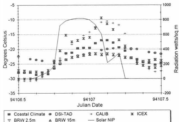
Fig. 2. Hourly-averaged temperature readings for four buoys and the BRW standards. Direct solar radiation is shown by measurements from the Normal Incidence Pyrometer (NIP). The effects of solar heating are depicted.
