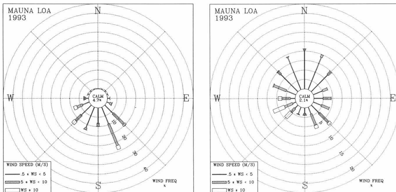
Fig. 4.3. Wind roses of the surface winds for MLO for 1993 night (left) and day (right). The distribution of resultant wind direction and speed are given in units of percent occurrence for the year. Wind speed is displayed as a function of direction in three speed classes.
