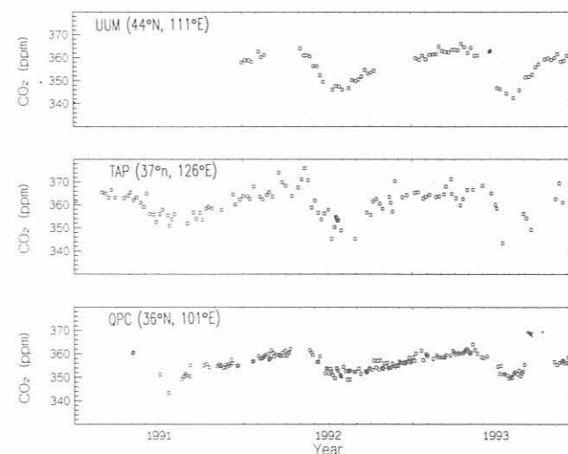
Fig. 2.3. CO 2 mixing ratios determined for flask samples collected at Ulaan Uul, Mongolia (UUM); Tae-ahn Peninsula, South Korea (TAP); and Qinghai Province, China (QPC) from 1991 through 1993. The square symbols represent the average CO 2 mixing ratios for two flasks collected in series.
