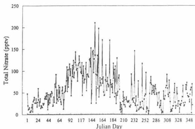
Fig. 1. Nightly concentrations of total nitrate in 1993.
