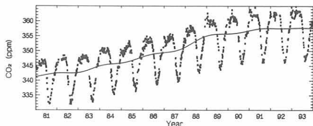
Fig. 2.4. \text{CO}_2 mixing ratios measured in flask samples collected at Mould Bay, Canada (MBC). The square symbols represent the average value for two flasks collected in series. The smooth curve represents the deseasonalized long-term trend. Note the near-zero increase in 1992 and the slight increase in 1993.
