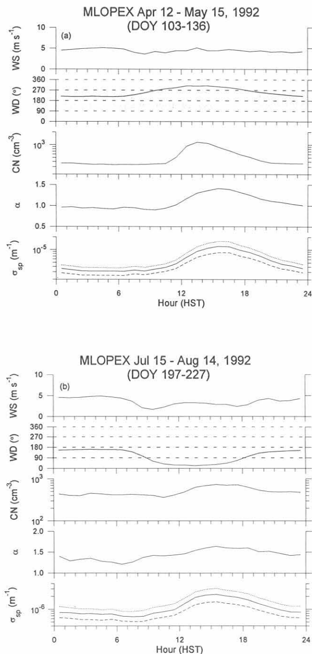
Fig. 3.21. Data for MLOPEX (a) intensive 3 and (b) intensive 4. Means by hour are shown for wind speed (WS); wind direction (WD); CN concentration; \alpha ; and \sigma_{sp} for 450 (dotted), 550 (solid), and 700 nm (dashed). \alpha values were calculated using equation (1). The shaded areas on the WD graphs denote winds with a southerly (downslope) component. Hour of the day is shown as HST.
