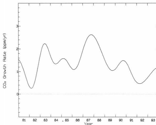
Fig. 2.6. The globally averaged \text{CO}_2 growth rate obtained from the flask network data. Because this curve is based on data only through the end of 1993, the last 6 months must be viewed with caution. Preliminary 1994 data suggest that the upturn of the growth rate in 1993 will continue into 1994.
