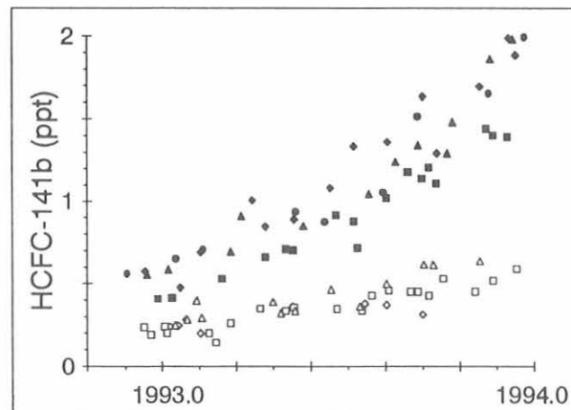
Fig. 5.10. Mixing ratios determined for HCFC-141b from air collected in flasks from seven different remote sampling locations: Alert, (•); BRW, (Δ); Niwot Ridge, (◆); MLO, (■); SMO, (Δ); CGO, (□); and SPO, (◇).
