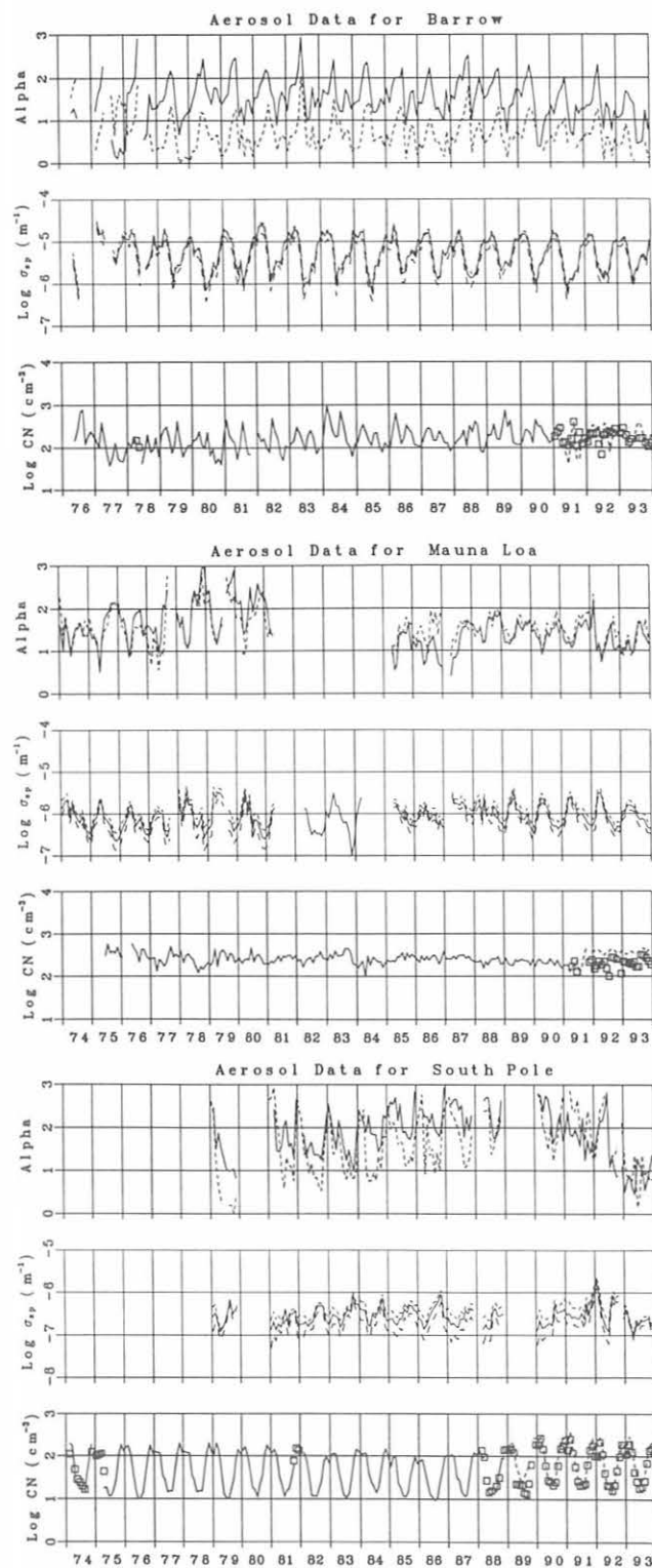
Fig. 3.2. Monthly geometric means of \sigma_{sp} and CN data for the entire data record at BRW, MLO, and SPO. Data for MLO are included only for 0000-0800 HST. \sigma_{sp} data (middle) are shown for 450 (dotted), 550 (solid), and 700 nm (dashed). Angstrom exponents (alpha) were calculated from 450 and 550 nm (dotted) and 550 and 700 nm (solid) \sigma_{sp} data. Note that G.E. CN counter data are shown as a solid line, TSI CN counter data are shown as a dashed line, and Pollak CN counter data are shown as small squares.
