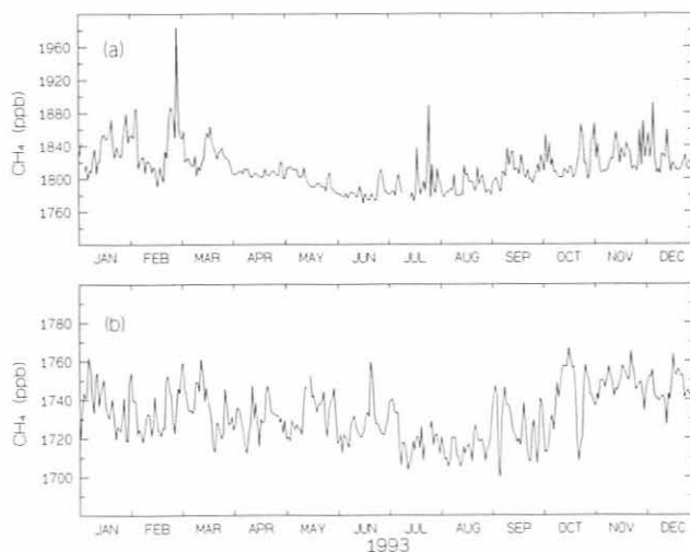
Fig. 2.8. Daily mean \text{CH}_4 mixing ratios in ppb for (a) BRW and (b) MLO for 1993. The data are unconstrained, but have undergone a quality control step to ensure that the analytical instrument was working optimally when they were obtained [Masarie et al. , 1991].
