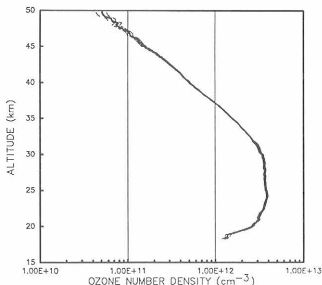
Fig. 1. MLO ozone profile for January 27, 1994.
