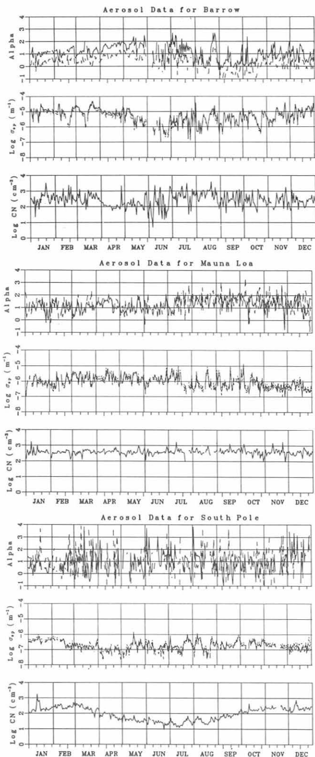
Fig. 3.1. Daily geometric means of \sigma_{sp} and CN data at BRW, MLO, and SPO for 1993. Data for MLO are included only for 0000-0800 HST. For each station, CN concentration data are shown as small squares. \sigma_{sp} data (middle) are shown for 450 (dotted), 550 (solid), and 700 nm (dashed). Angstrom exponents (alpha) were calculated from 450 and 550 nm (dotted) and 550 and 700 nm (solid) \sigma_{sp} data.
