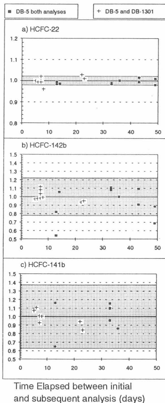
Fig. 5.11. Results obtained when air within samples flasks was re-analyzed after a period of time had elapsed for (a) HCFC-22, (b) HCFC-142b, and (c) HCFC-141b. Squares represent re-analyses that were performed under identical instrumental conditions. Plus symbols (+) represent results from re-analyses that were performed with a more polar analytical column (DB-1301 versus DB-5). The shaded area represents 2 times 95% of the range of variability observed for duplicate injections of air from all flasks collected in 1992 and 1993.
