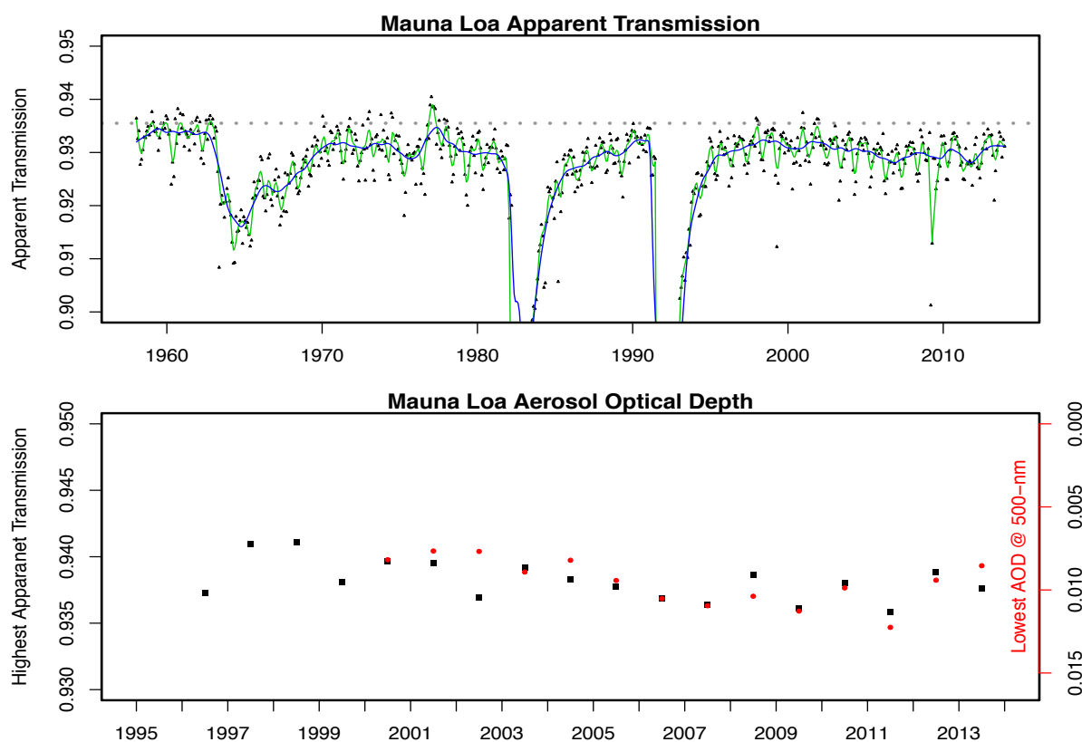
Fig. 7-9: Top: Monthly mean of the clear-sky Apparent Transmission at MLO. Means are determined from the early morning values. The green line is the 6-month running smoothed fit, and the blue line is the 24-month smoothed fit using only monthly means that include at least ten days. The dashed line is the background level from 1958 – 1972. Bottom: Annual averages of the 10 cleanest days of the year for the clear-sky Apparent Transmission (black squares) and the aerosol optical depth from a collocated PFR (red dots).
