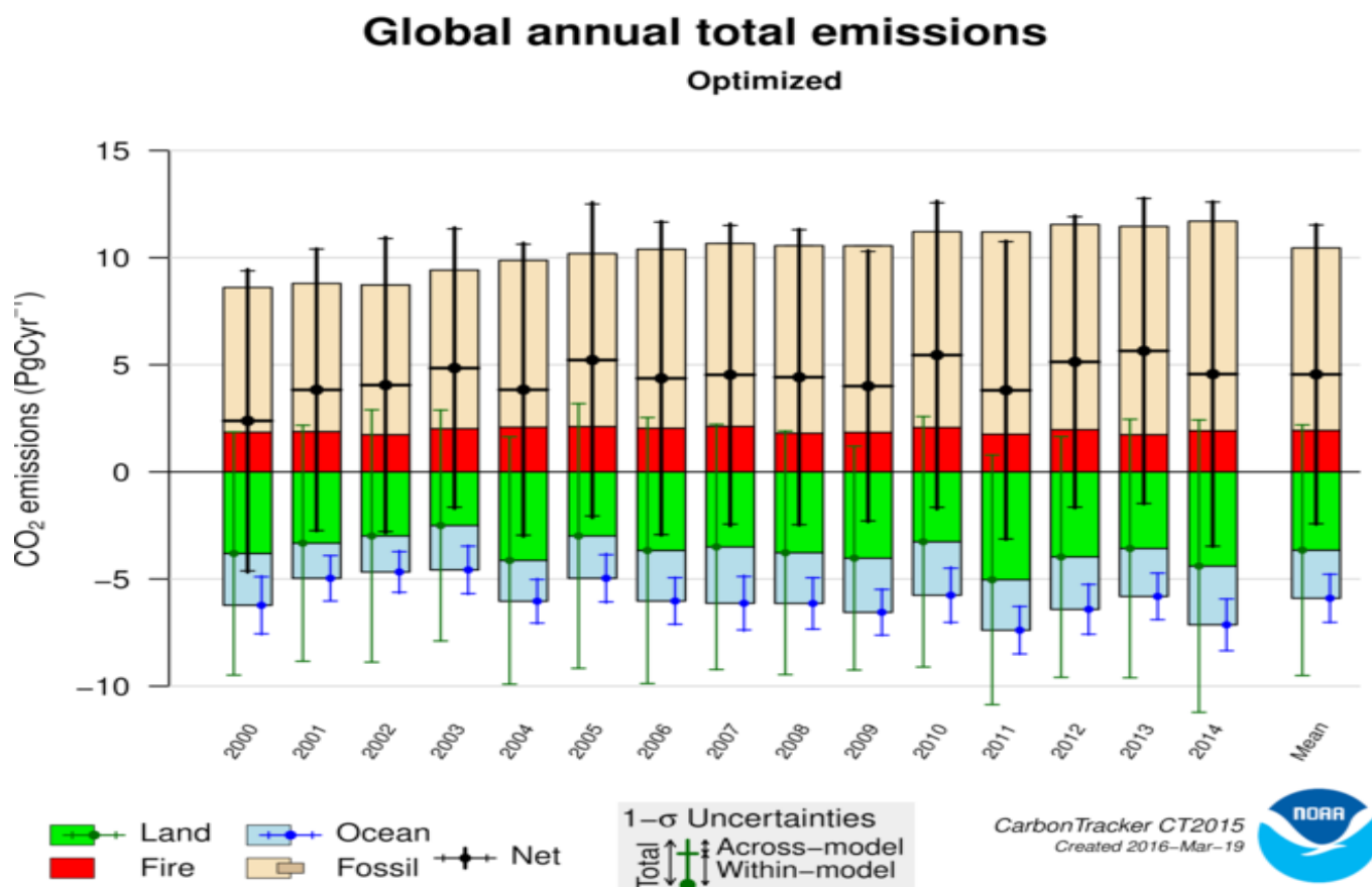
Fig. 4-3: Estimated global emissions by the CarbonTracker data assimilation system by source category. Fire and fossil fuel plus cement emissions are specified by inventories, while ocean and land sources are solved for by CarbonTracker, based on atmospheric CO 2 observations. The total net annual source to the atmosphere (thick black lines) corresponds very closely to the observed global annual averages that we derive from Marine Boundary Layer sampling sites ( http://www.esrl.noaa.gov/gmd/ccgg/trends/global.html ).
