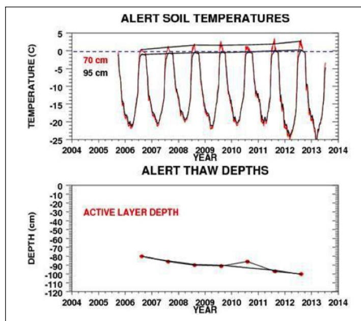
Fig. 7-7: Time series of 12-hour resolved soil temperatures at ALT at the 70 cm and 95 cm depths where the peak thaw occurs during summer. The active layer depth (ALD) typically falls within the 70–95 cm depth range (bottom). Estimates of ALD for the years of available data (2005–2012) are smoothed to show inter-annual and multi-year trend toward deeper thaw.
