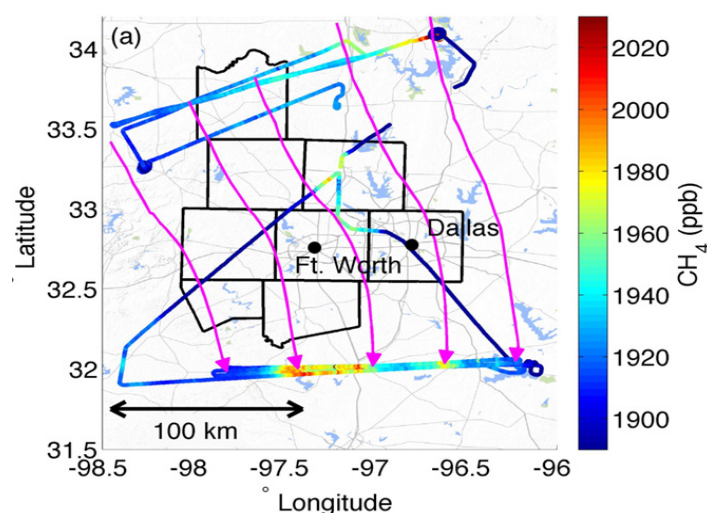
Fig. 4-5: Flight pattern on 19 October 2013 over the Barnett Shale oil and gas field for “mass balance” estimation of total methane leaks from the area. The downwind enhancement of the \text{CH}_4 mole fraction and the wind speed and direction (pink arrows from northwest veering toward south), as well as the boundary layer height are used. There were multiple transects downwind at different altitudes.
