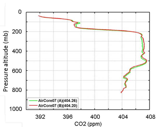
Fig. 4-8: Vertical profiles of \text{CO}_2 in two different AirCores flown simultaneously to an altitude of 28 km.
