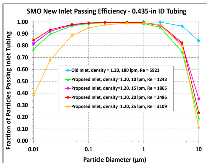
Fig. 3-4: Particle passing efficiency curves for the old SMO inlet compared with several flow rates through the new inlet.
