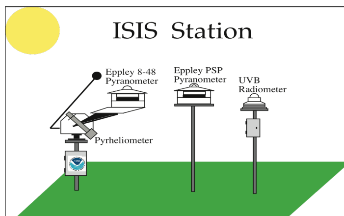
Fig. 7-1: Complement of instruments at each ISIS network station. Downwelling radiation only is measured at these sites.
