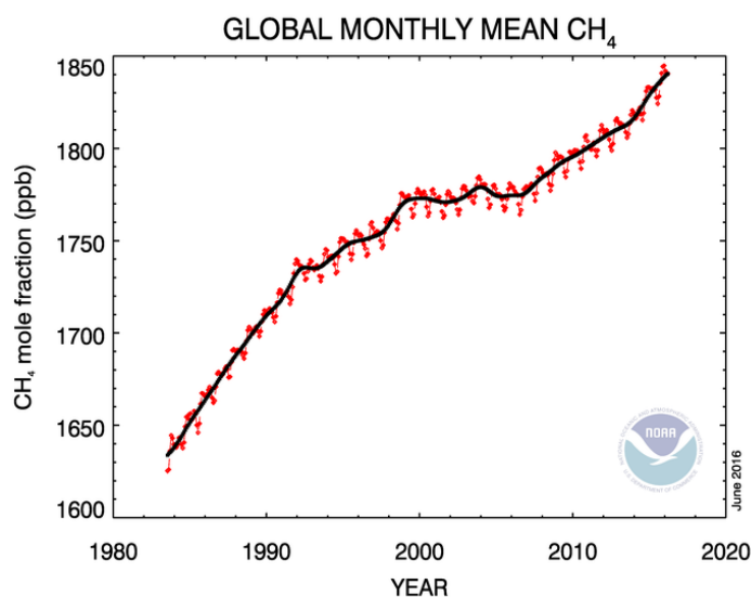
Fig. 4-1: Globally averaged monthly averages (red) and long term trend (black) of methane. The global average is based on the Marine Boundary Layer sites, a subset of the global cooperative flask air sampling network consisting of sites with access to well mixed surface air that has been over the oceans for weeks ( http://www.esrl.noaa.gov/gmd/ccgg/trends_ch4/ or see section 4.3 Data Products).
